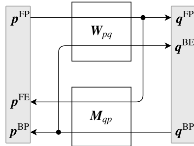
Fig. 1: UBAL connectivity of two connected layers \mathbf{p} and \mathbf{q} .
